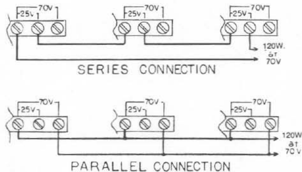
FIGURE 2: OUTPUT CONNECTIONS FOR PARALLEL OR SERIES OPERATION.
